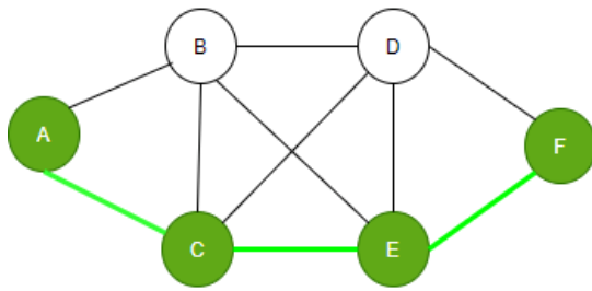
UnWeighted Graph
