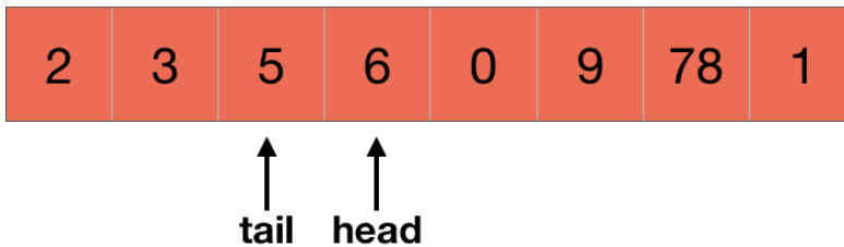
Queue Overflow
